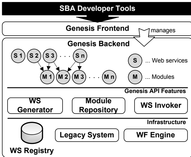
Figure 4: Architectural overview.
